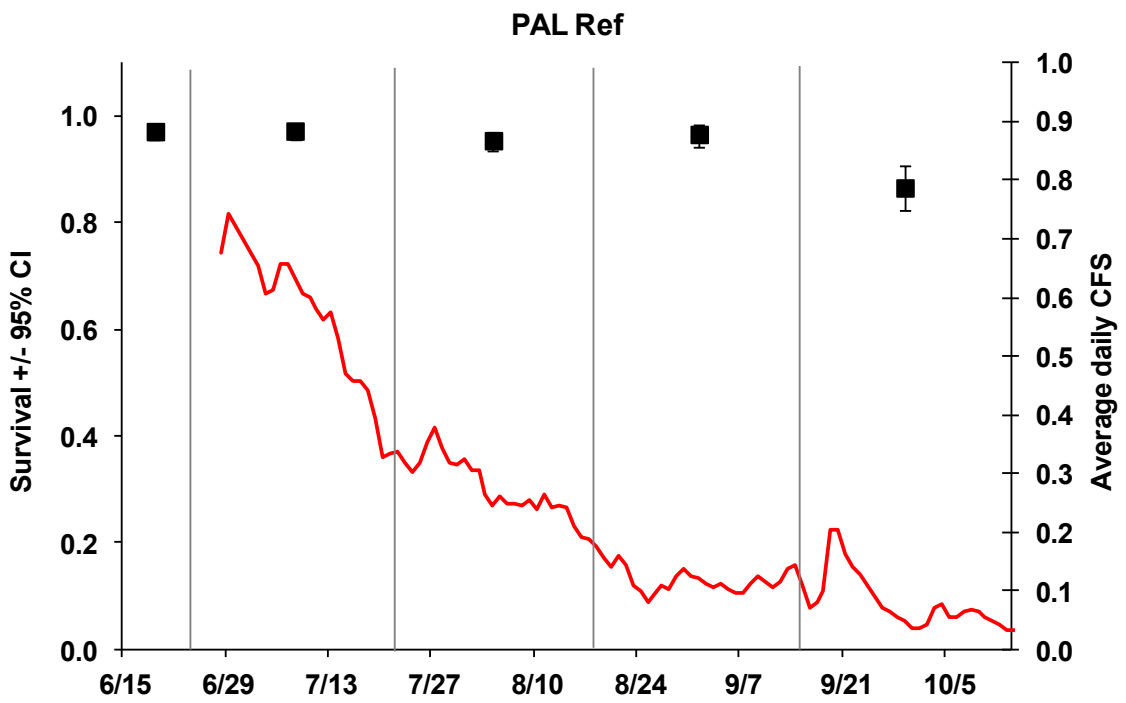
Figure 29. Monthly survival of coho yoy released into the Palmer Creek reference reach in relation to stream flow. Gray bars represent PIT tag wand sampling occasions.
