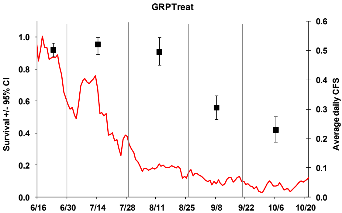
Figure 30. Monthly survival of coho yoy released into the Grape Creek treatment reach in relation to stream flow. Gray bars represent PIT tag wand sampling occasions.
