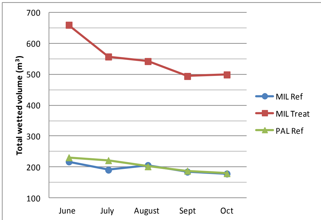
Figure 7. Total wetted volume of pool and flatwater habitat in Mill Creek and Palmer Creek reference and treatment reaches between June and October, 2010.
