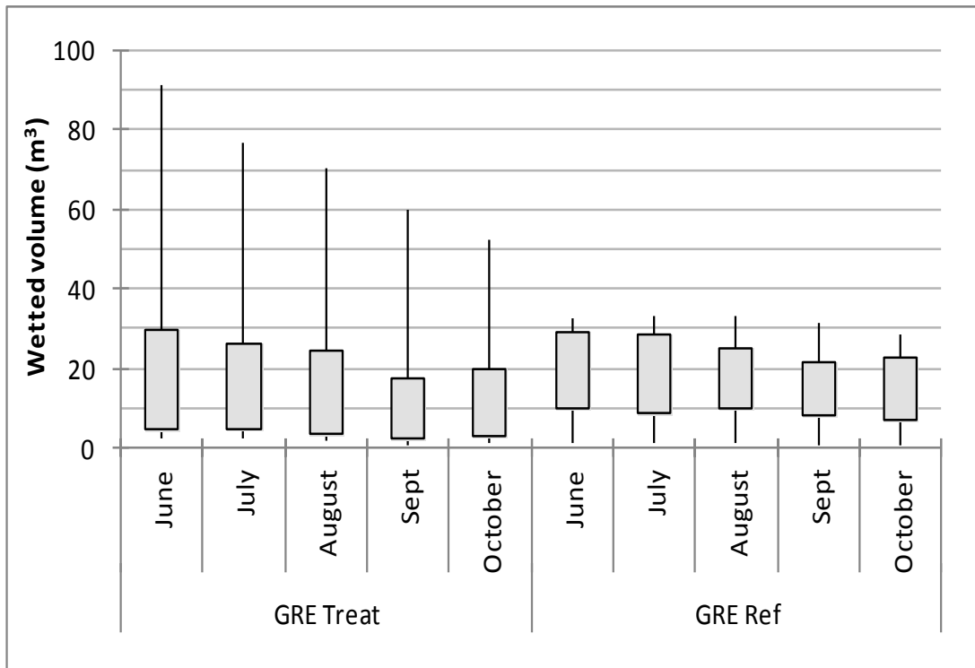
Figure 9. Minimum, maximum, 25 percentile, and 75 percentile of average wetted volume of pool and flatwater habitat in Green Valley Creek reference and treatment reaches between June and October, 2010.
