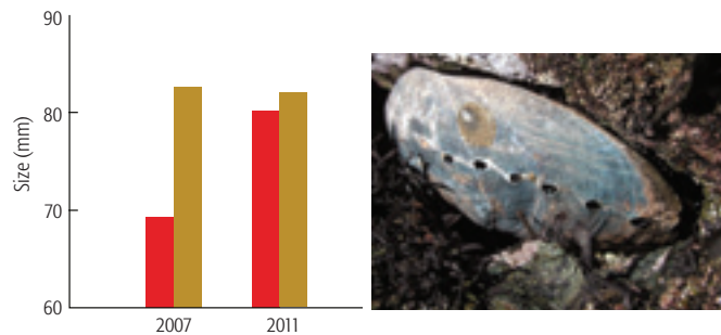
Average changes in the size of owl limpets (upper) and black abalone (lower) between 2007 and 2011 inside State Marine Reserves (SMR) and outside at comparable reference points. Source: PISCO, UCSC
